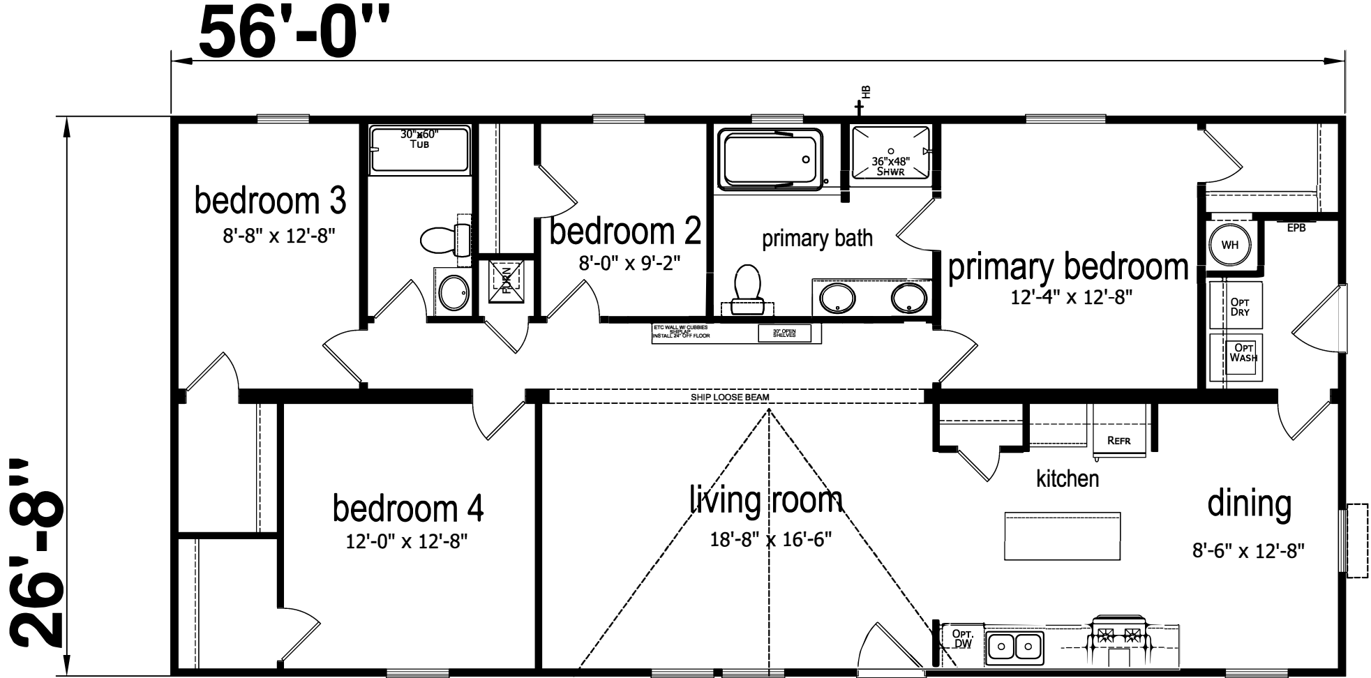
21-2856H42LM56-4COM Ranger 4 BEDROOM 2 BATH 56'-0" x 26'-8" TOTAL AREA: 1493 SQ. FT.
